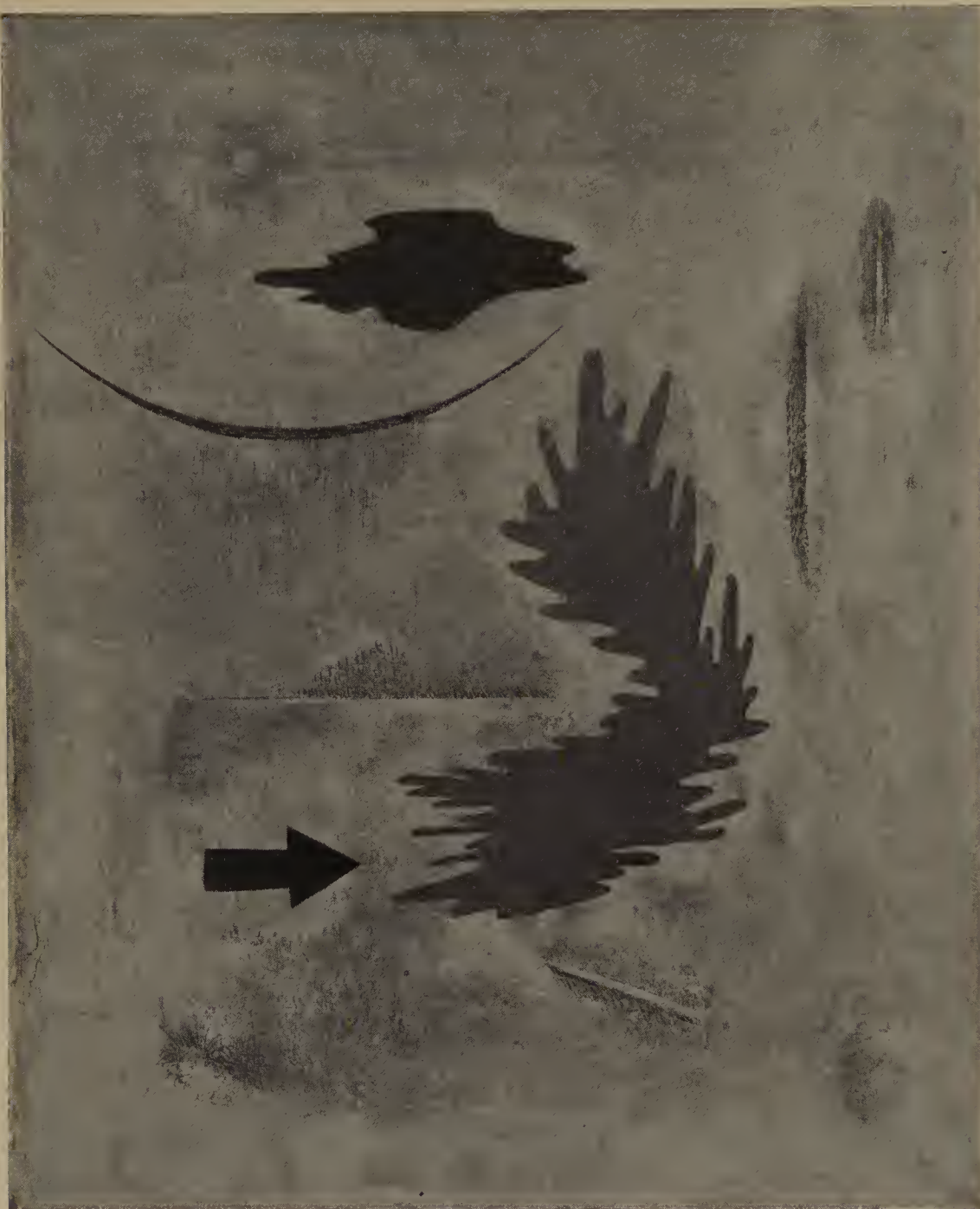
The water cycle
