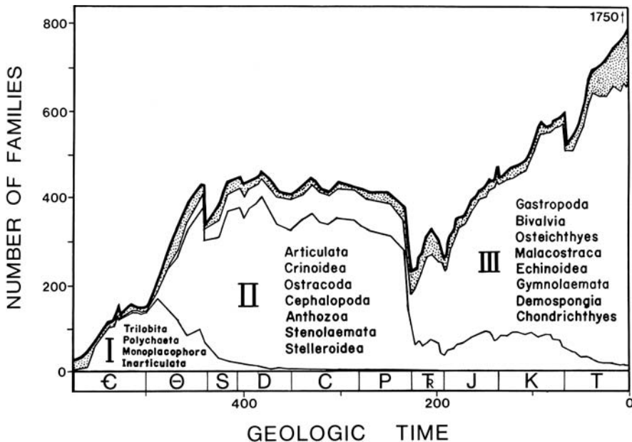
Fig. 2.8 Jack Sepkoski's three-curve graph of Phanerozoic marine faunal diversity, in J. John Sepkoski, Jr., "A Kinetic Model of Phanerozoic Taxonomic Diversity: III. Post-Paleozoic Families and Mass Extinctions," Paleobiology 10 (1984).
