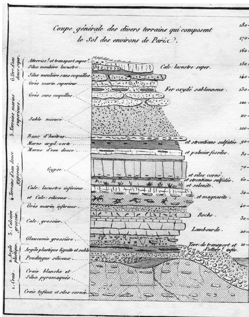
Fig. 2.1 Cuvier and Brongniart's idealized strata of the Paris basin, in Cuvier, Ossements fossiles (Paris, 1812).
